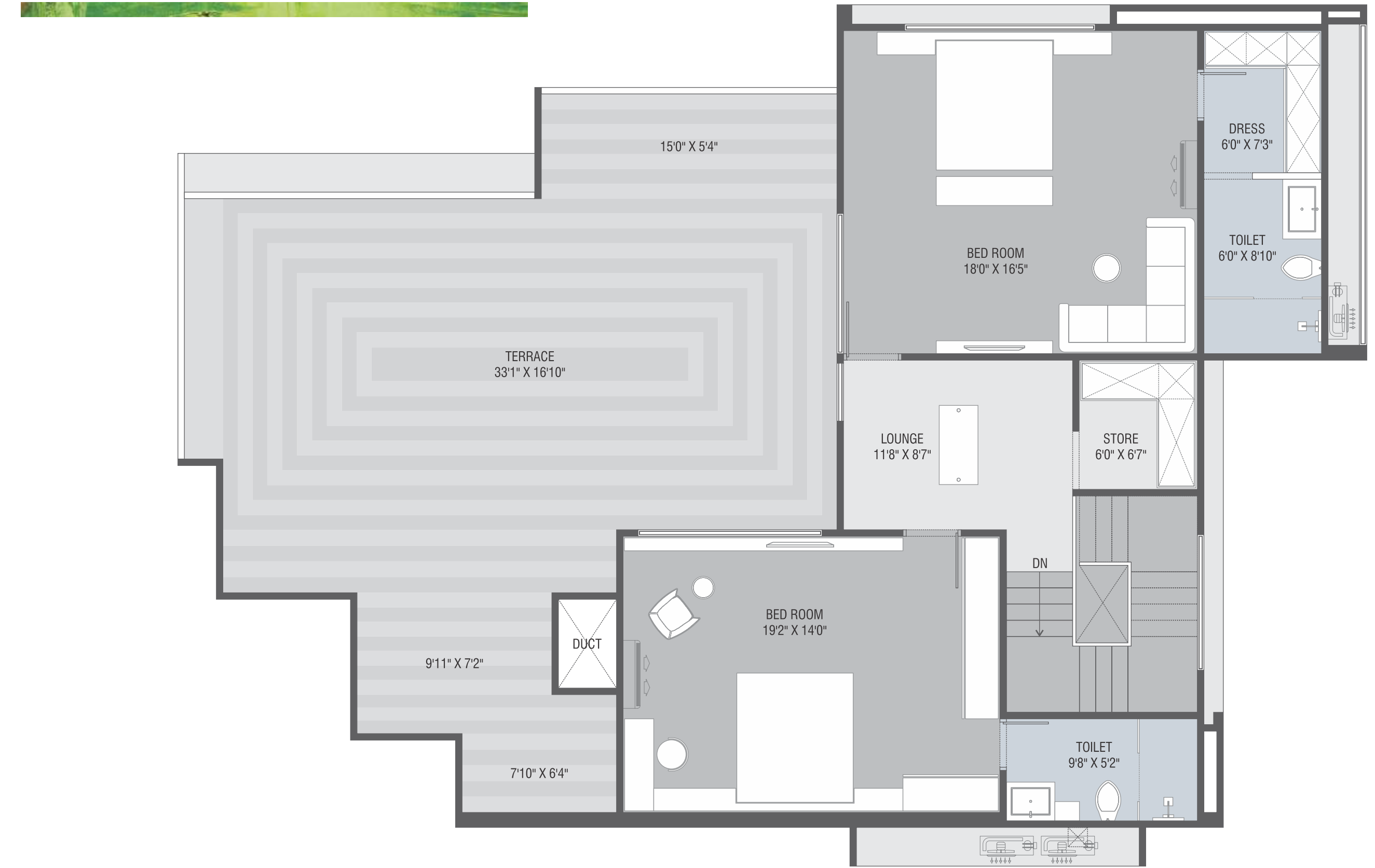
14 th floor plan (5bhk pent house-upper level)
